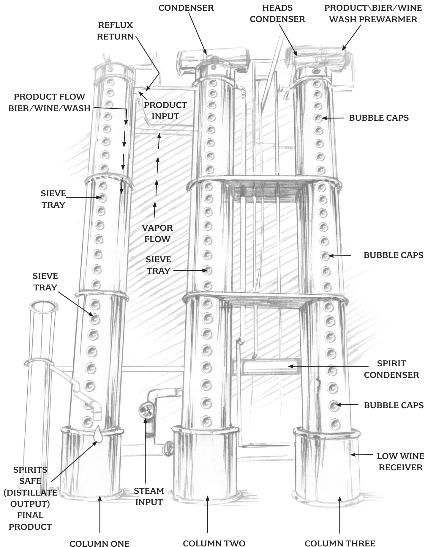
MONSON RANCH DISTILLERY'S STILL
