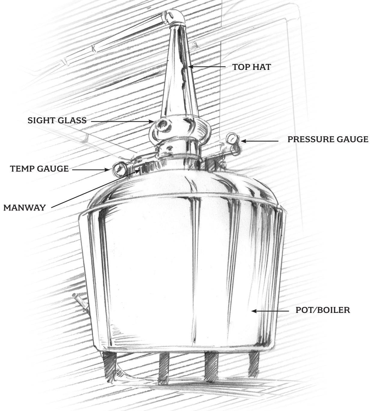
MONSON RANCH DISTILLERY'S POT STILL
